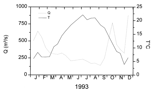
Fig. 2. A characteristic annual cycle of discharge (Q in \text{m}^3/\text{s} ) and water temperature ( T^\circ\text{C} ) of the Seine river measured at Poses. Year 1993.
