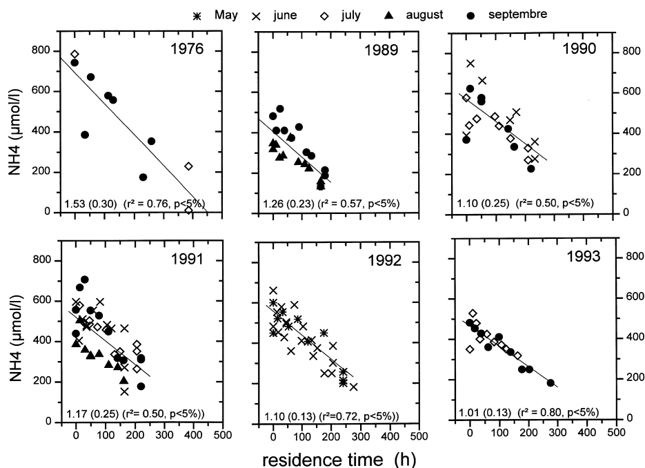
Fig. 6. Ammonium concentration ( \text{NH}_4 in \mu\text{mol/l} ) profiles in the River Seine downstream of the Oise confluence at different stages in the history of Paris wastewater treatment. (A) 1976: Data from the A.E.S.N. (Agence de l'Eau Seine–Normandie). Very dry summer and about 1/4 of Paris effluents are still discharged without treatment. (B–F) 1989–1993: data from the A.E.S.N. Discharge of raw sewage is much reduced. Residence time of a water mass was calculated using discharge, wet sections and stream segment lengths values. It is set to 0 at the Oise confluence.
