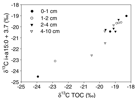
Fig. 8. Plot of \delta^{13}\text{C} signatures of bacterial PLFA ( i + a15:0 ) versus those of bulk sediment organic carbon in different depth sections of intertidal mangrove sediments from the Betsiboka estuary.
