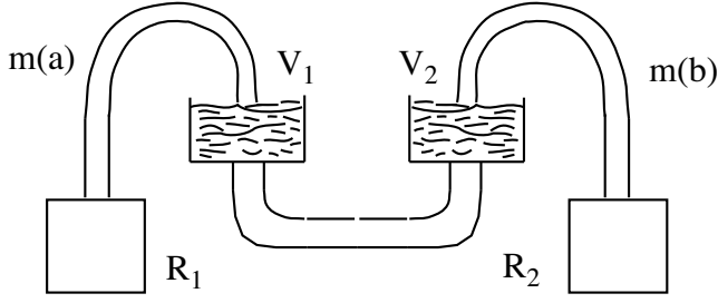
A classical macroscopical system that violates Bell-inequalities (fig 2).
