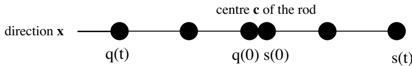
The system of two particles q and s bounded on a rigid rod in direction x , that move outwards, q to the left and s to the right (fig 5).
