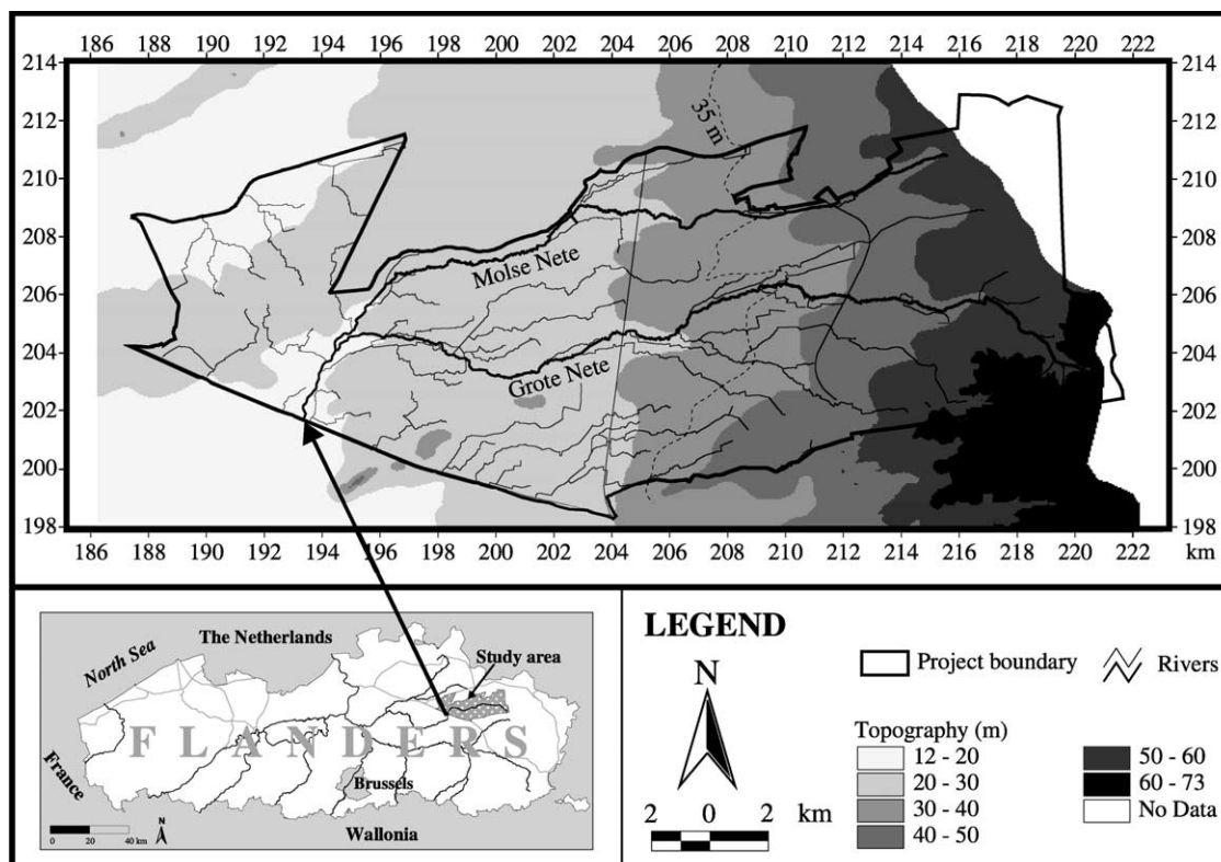
Fig. 1. Grote-Nete study area and topography.
