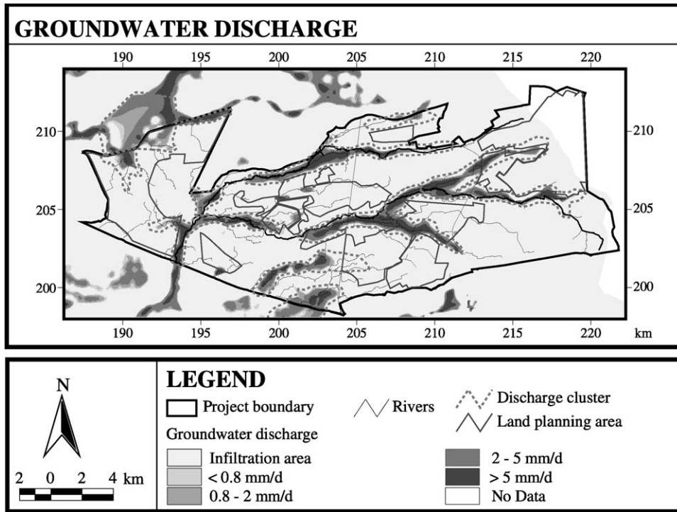
Fig. 6. Simulated groundwater discharge areas for the present situation.
