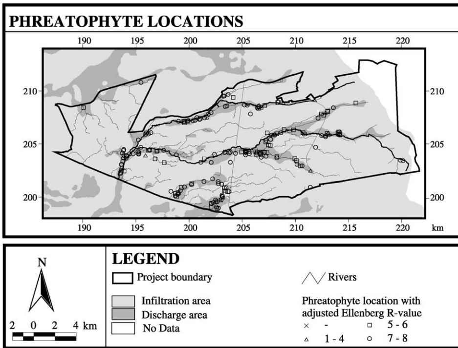
Fig. 9. Location of mapped phreatophytes and their weighted mean Ellenberg R-value, adjusted after Hill et al. (1999).
