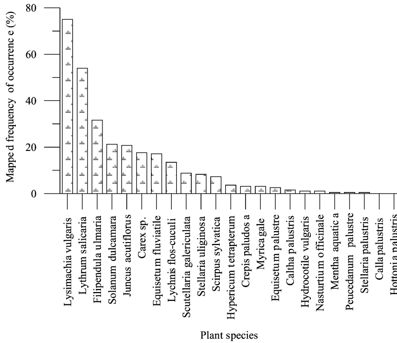
Fig. 8. Mapped frequency of occurrence of phreatophytic plant species.
