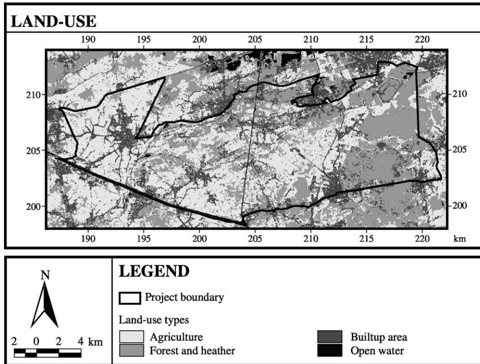
Fig. 2. Simplified land-use map for the Grote-Nete land planning project area (OC GIS-Vlaanderen, 1996).
