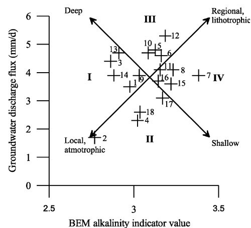
Fig. 13. Comparison of average BEM alkalinity indicator values with the groundwater discharge flux per groundwater discharge region. The clusters I (local, deep, upstream and atmotrophic), II (local, shallow, downstream and atmotrophic), III (regional, deep, central and lithotrophic) and IV (regional, shallow, downstream and lithotrophic) are indicated.
