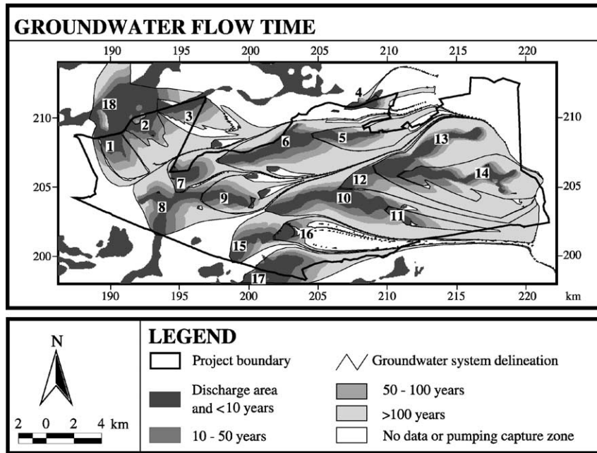
Fig. 10. Simulated groundwater flow systems for the present situation: the numbers (1–18) indicate the different discharge areas (for their delineation see Fig. 6), their contributing recharge areas are delineated by thin black lines, and the groundwater travel time from each recharge location to the indicated discharge location within a groundwater flow system is shown by means of grey scale contours.
