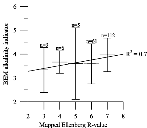
Fig. 11. Comparison of mapped Ellenberg R -values, adjusted after Hill et al. (1999), with corresponding BEM alkalinity indicator values (average and standard deviation are shown and the number of mapped locations is indicated).
