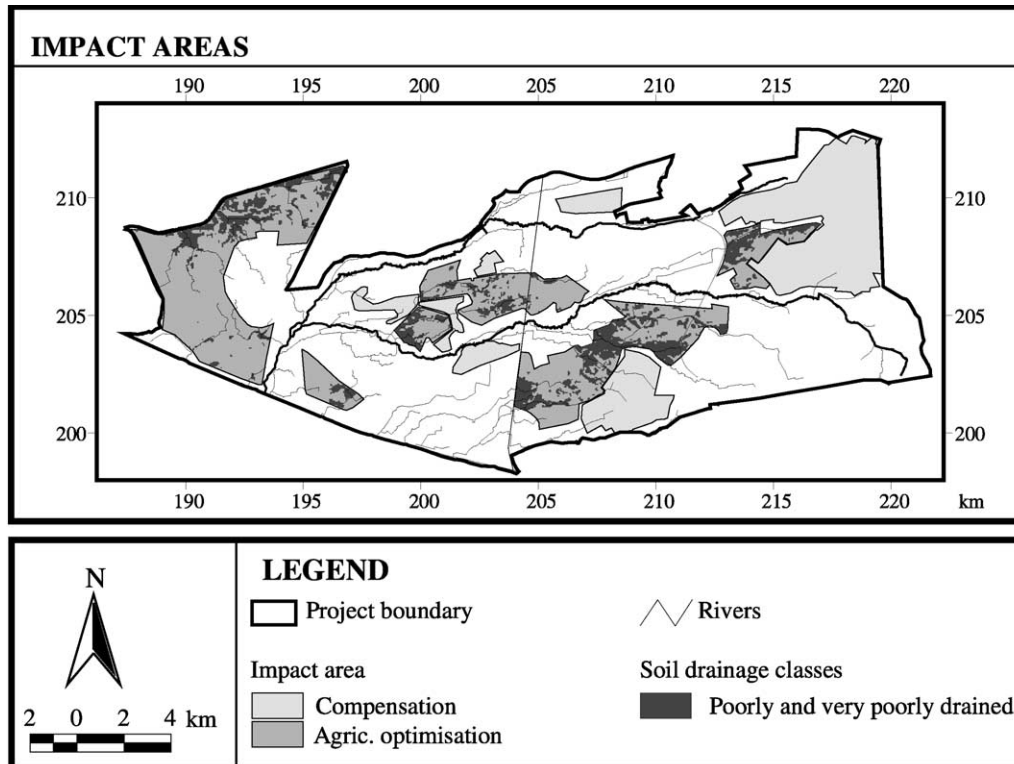
Fig. 3. Impact areas designated for agricultural improvement and compensation measures.
