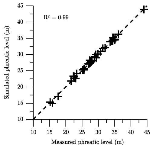
Fig. 7. Comparison of measured and calculated groundwater levels for Grote-Nete study area.
