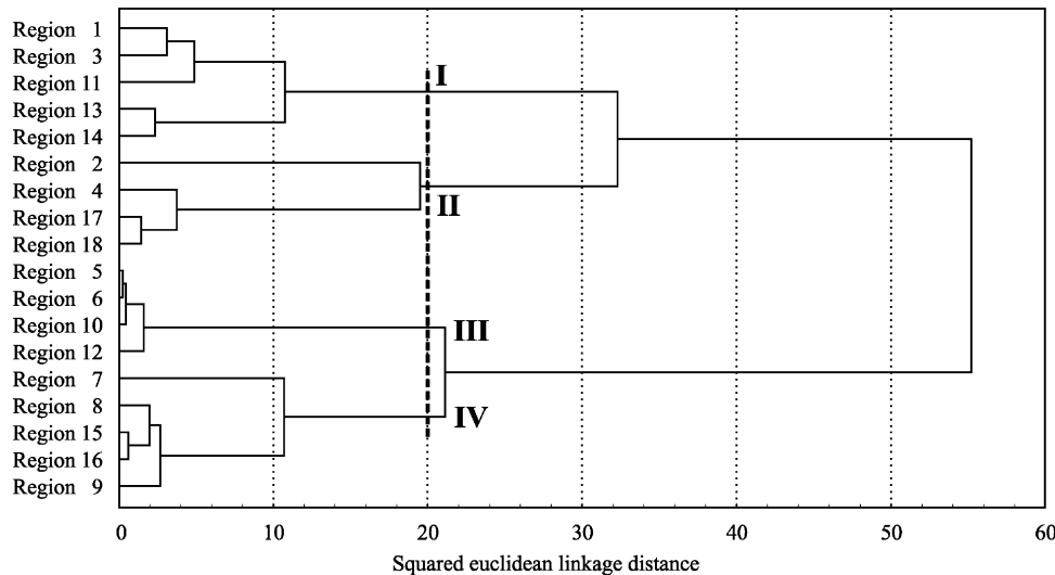
Fig. 12. Cluster dendrogram for the 18 groundwater flow systems.
