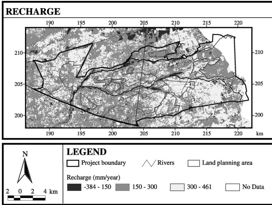
Fig. 4. Recharge for present situation calculated using WetSpss.
