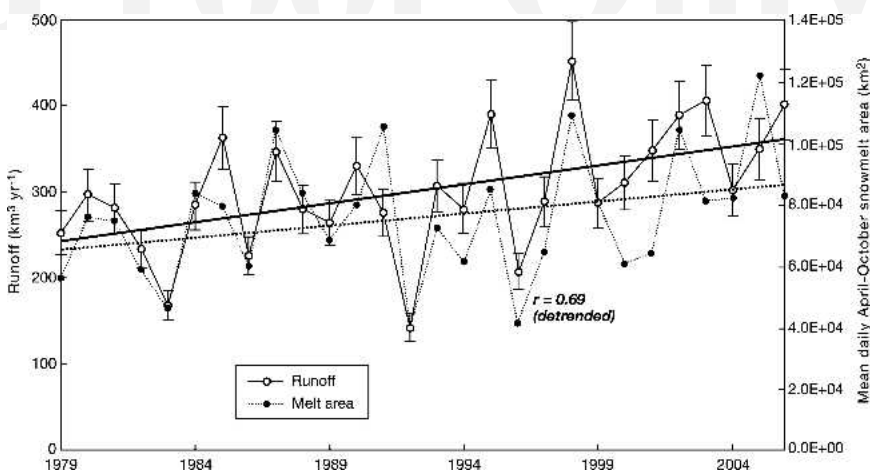
FIG. 6. Comparison of Greenland Ice Sheet annual runoff with satellite-derived snowmelt area, 1979–2006.
